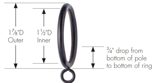
CORIM100 1" Metal Ring
