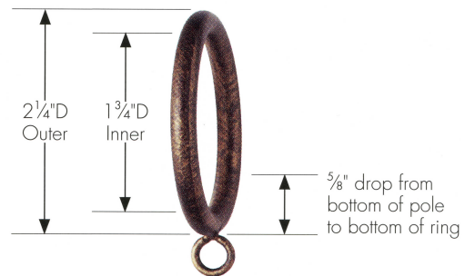
CORIM138 1 3/8" Metal Ring
